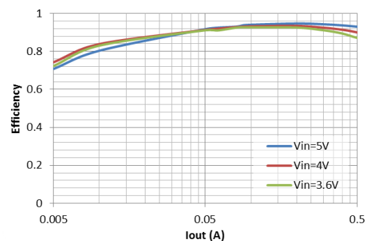
ETA1611 12V output efficiency
